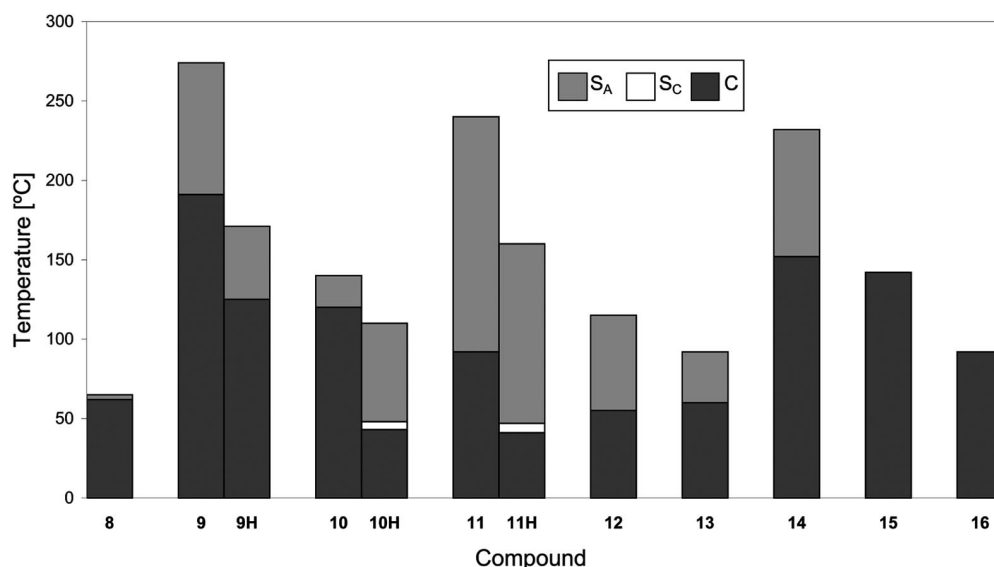
Figure 4. Graphical comparison of phase-transition temperatures for ligand 8 , complexes 9–16 , and their hydrocarbon analogues (labeled with suffix H ).
