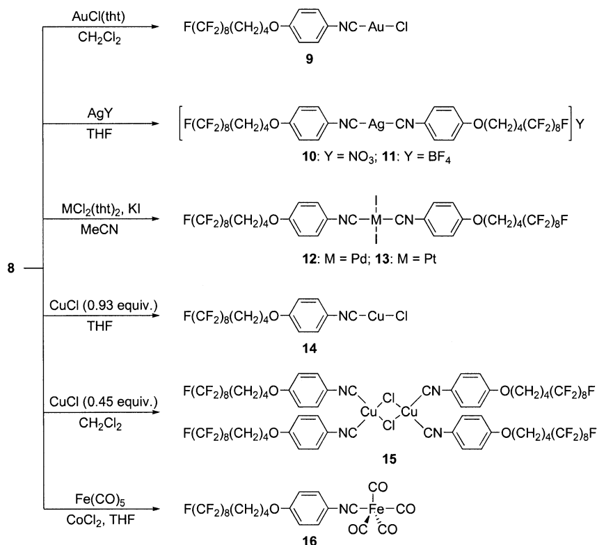
Scheme 2. Preparation of complexes 9–16 (tht = tetrahydrothiophene).
