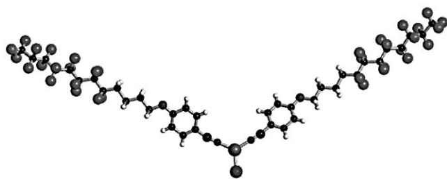
Figure 2. Molecular structure for copper complex 15 . Monoclinic, C2/c , a/b/c = 20.994(3)/6.1438(9)/35.104(5) Å, \beta = 93.571(2)^\circ , Z = 4 . Selected interatomic distances [Å]: Cu1–C1 1.895(4), Cu1–Cl1 2.2086(16). Key angles ^\circ : C1–Cu1–C1' 125.1(2), C1–Cu1–Cl1 117.46(12), N1–C1–Cu1 176.2(4).
