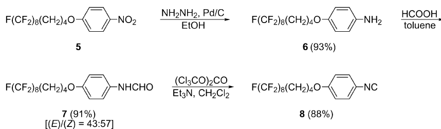
Scheme 1. Synthetic route to fluorous isocyanide 8 .
