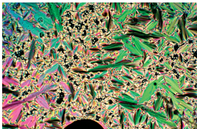
Figure 3. Polarized-light optical photomicrograph of the fan-shaped texture of the smectic A phase on cooling of 8 at 50^\circ\text{C} .
